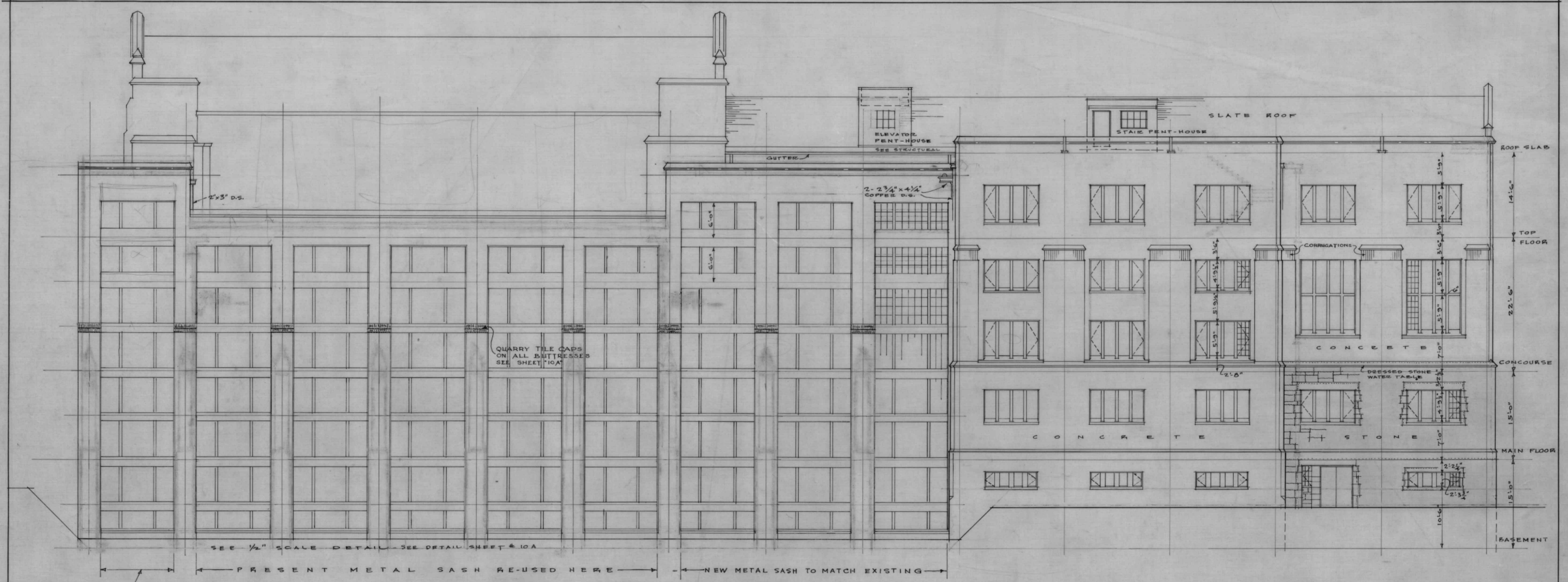
REAR (EAST) ELEVATION
