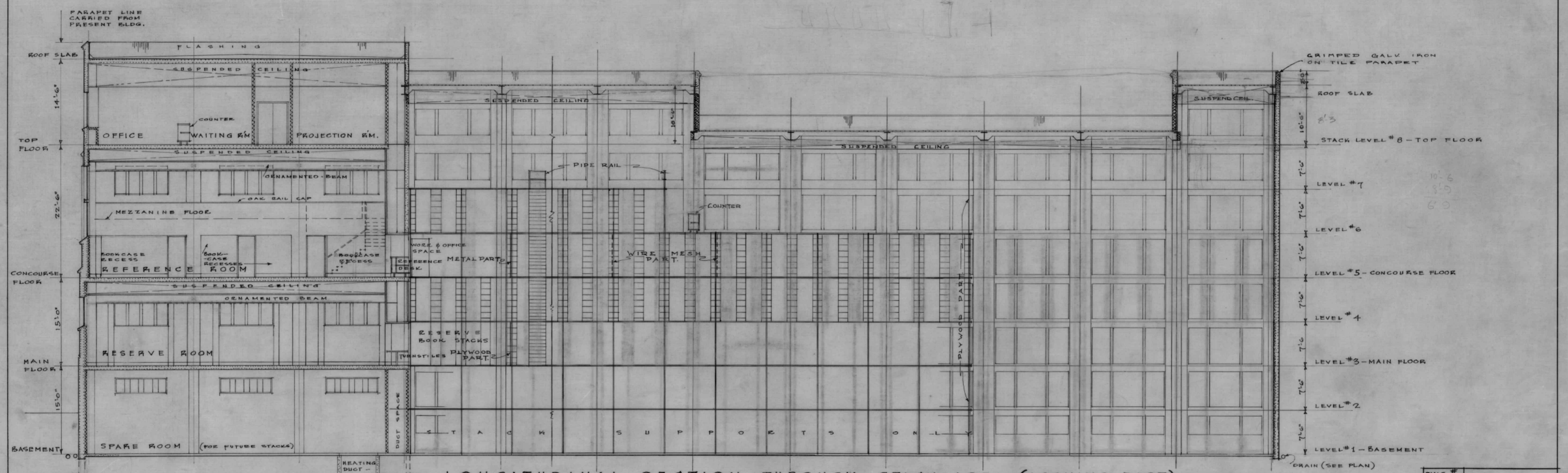
LONGITUDINAL SECTION THROUGH STACK AREA (LOOKING EAST)
